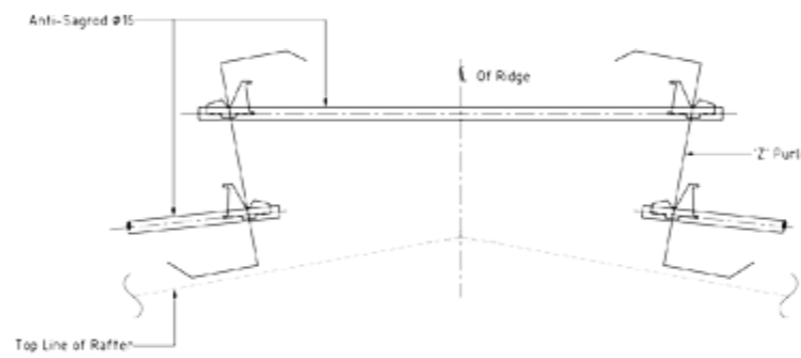
Anti-Sag rod Detail (Quick Lock System) (At Ridge)
